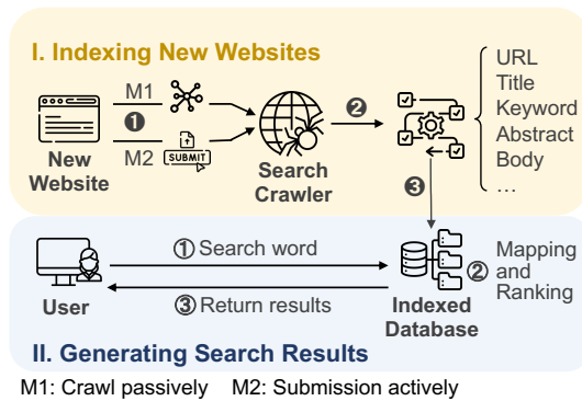
Figure 3: Indexing process of search engine for a new website and returning search results for users.
