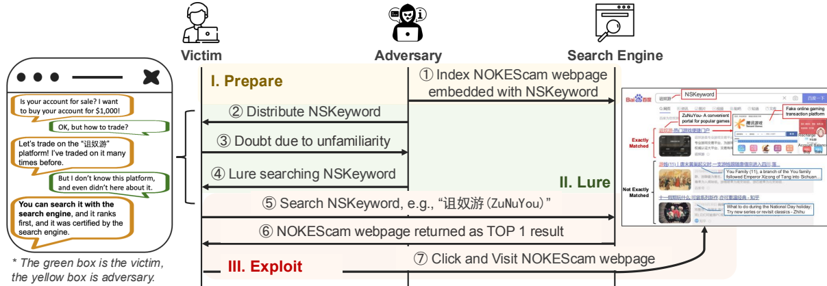
Figure 2: Workflow of NOKEScam.
