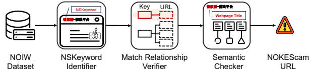
Figure 4: Workflow of our detection system for NOKEScam.
